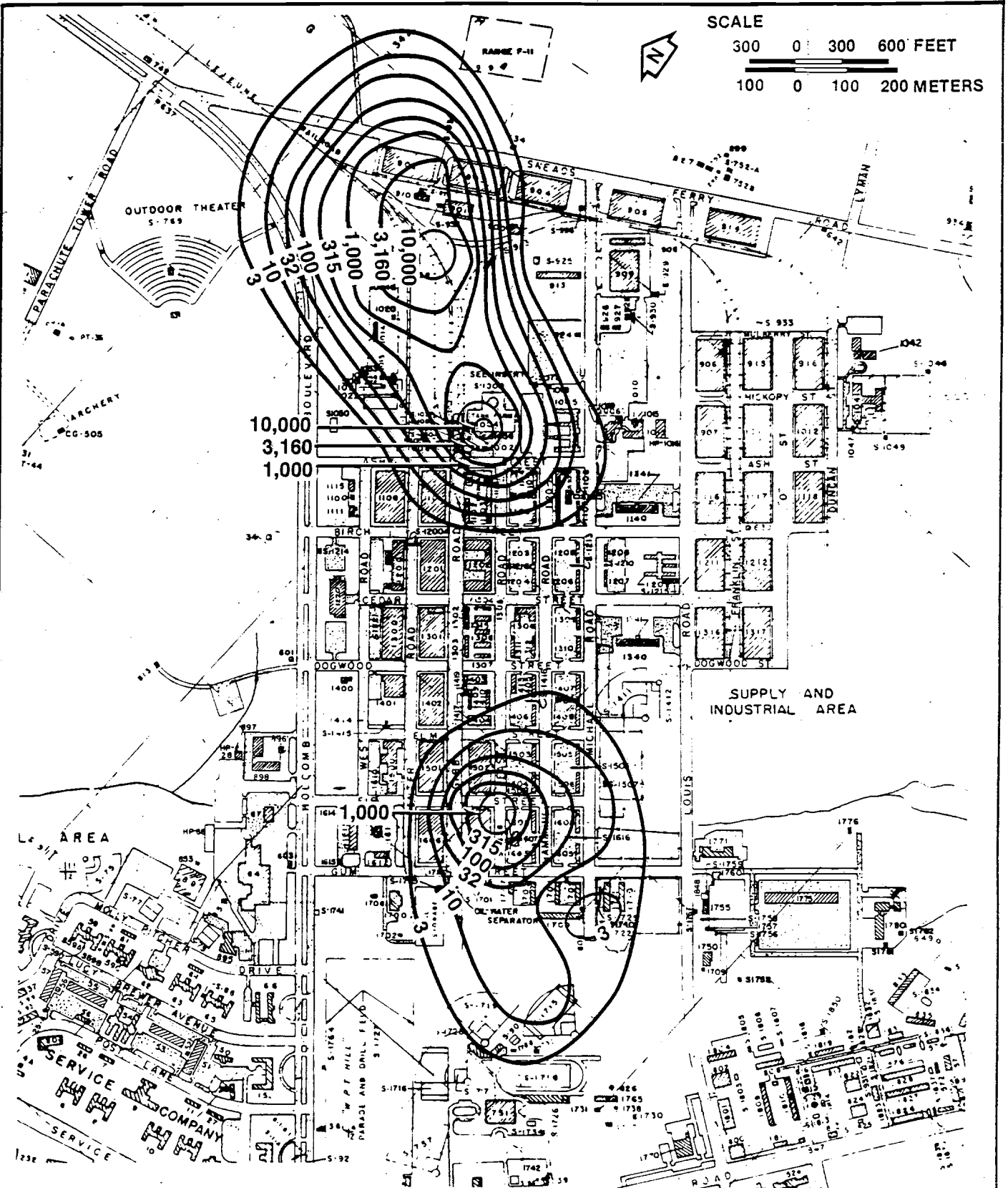
Figure 2-2 TOTAL VOLATILE ORGANIC COMPOUND ISOPLETH MAP — HADNOT POINT INDUSTRIAL AREA SOURCE: ESE, 1987.
