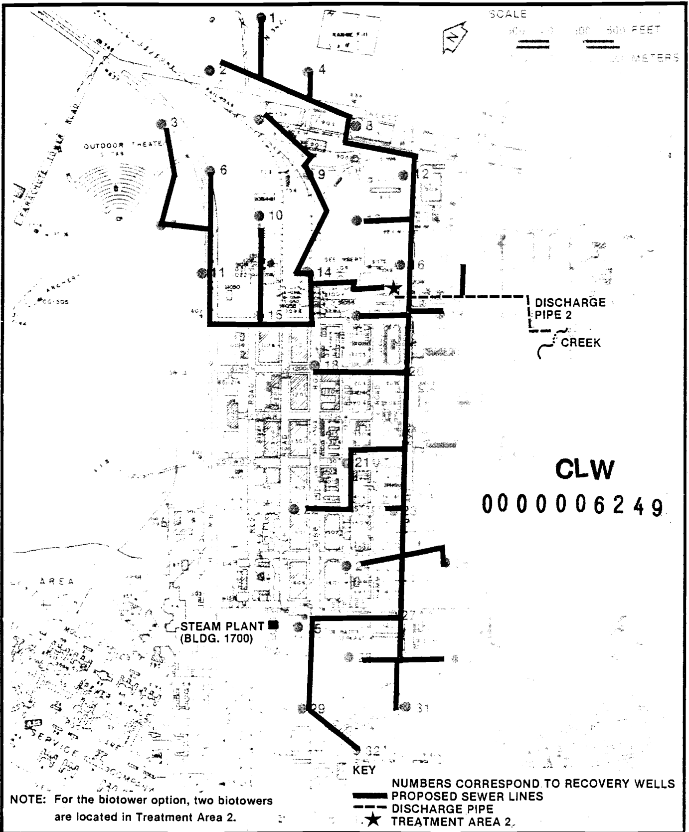
Figure 6-6 PIPING DIAGRAM FOR ALTERNATIVE 2 — (PACKAGE BIOLOGICAL TOWERS), ALTERNATIVE 4 (AIR STRIPPING), AND ALTERNATIVE 5 (STEAM STRIPPING) SOURCE: ESE, 1987.
