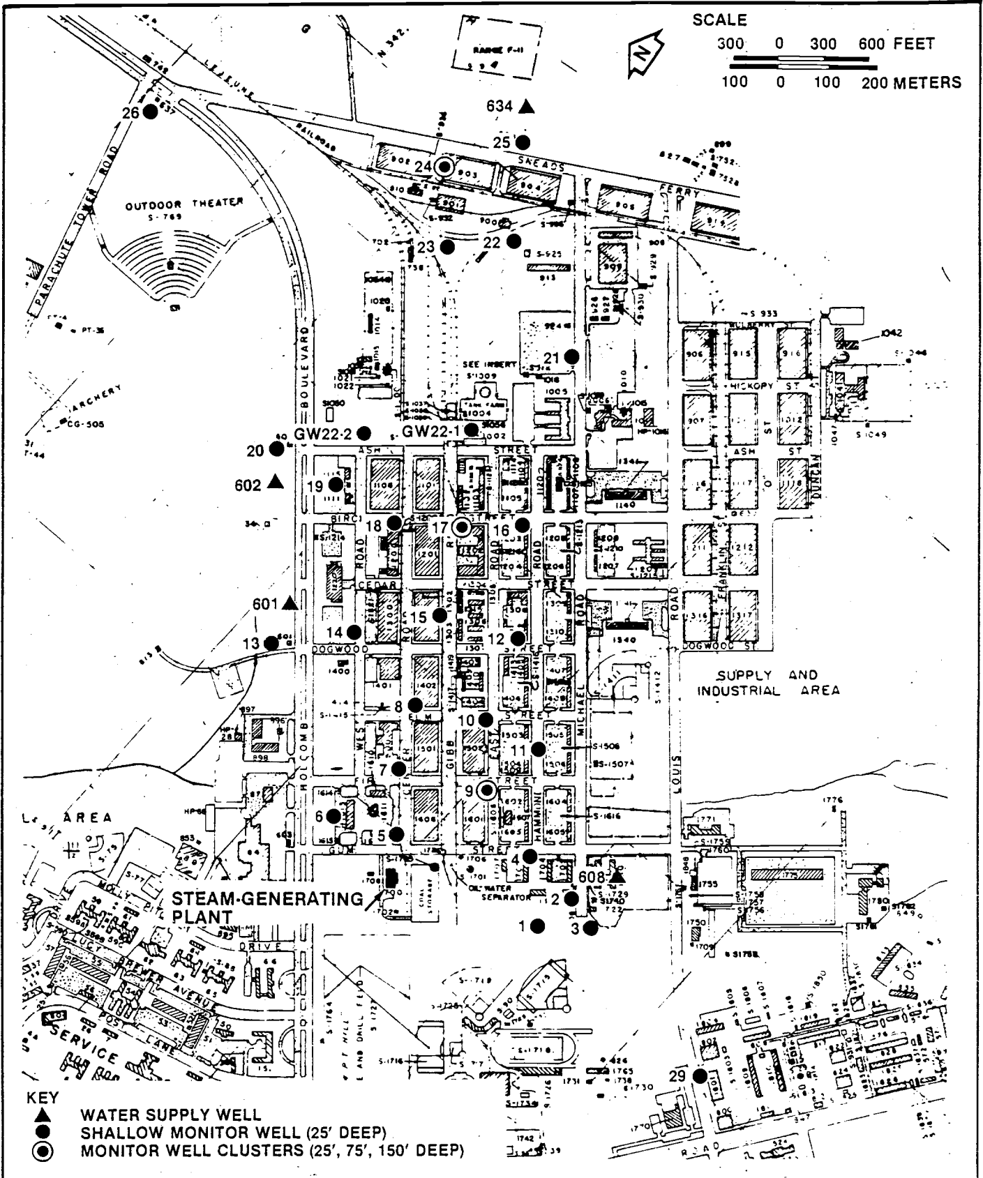
Figure 2-1 LOCATION OF MONITOR WELLS AT HADNOT POINT INDUSTRIAL AREA INSTALLED AFTER SOIL GAS INVESTIGATION SOURCE: ESE, 1987.
