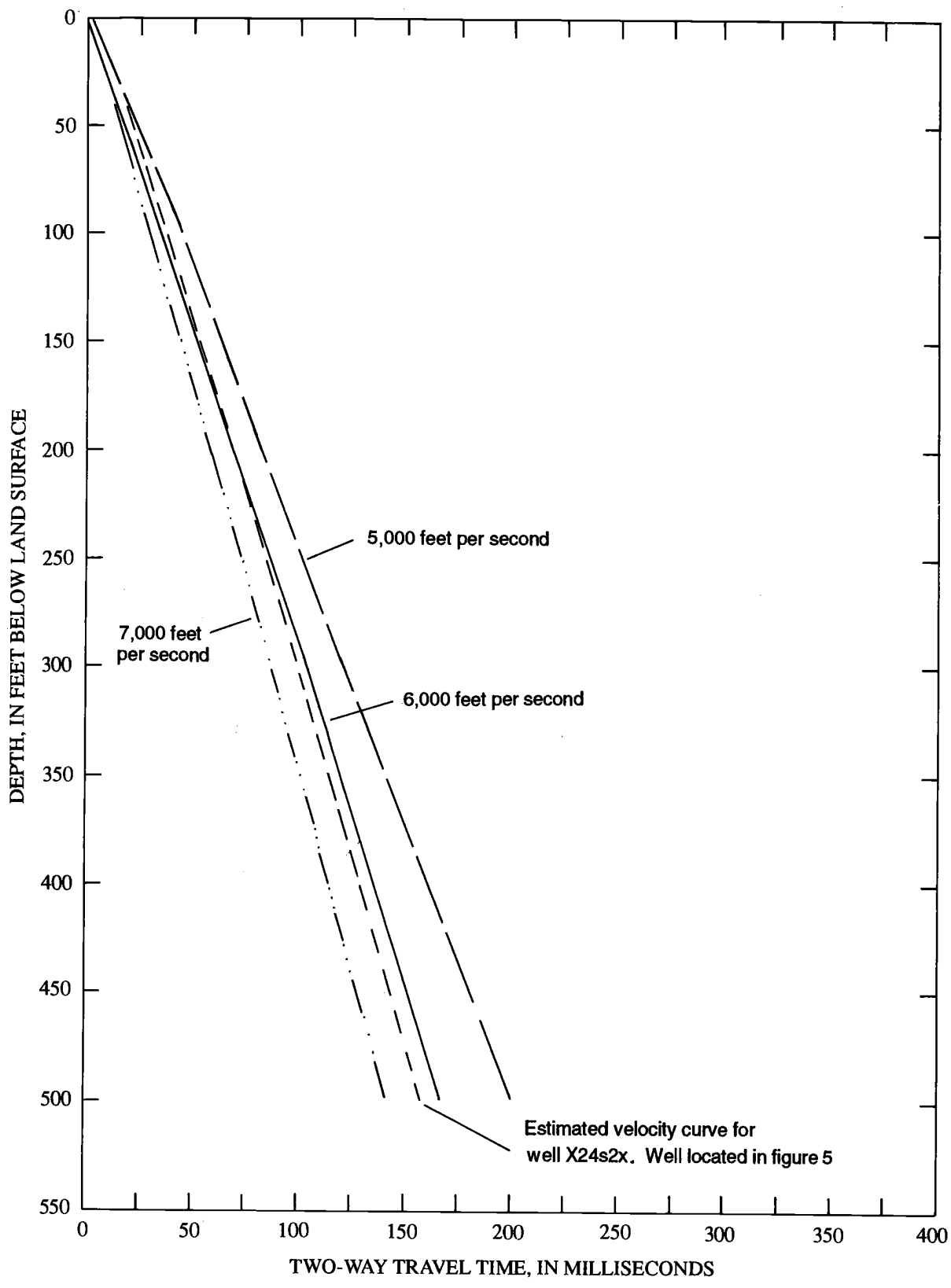
Figure 6.--Average acoustic-velocity curve for sediment at well X24s2x, Camp Lejeune, North Carolina (modified from Cardinell and others, 1990).
