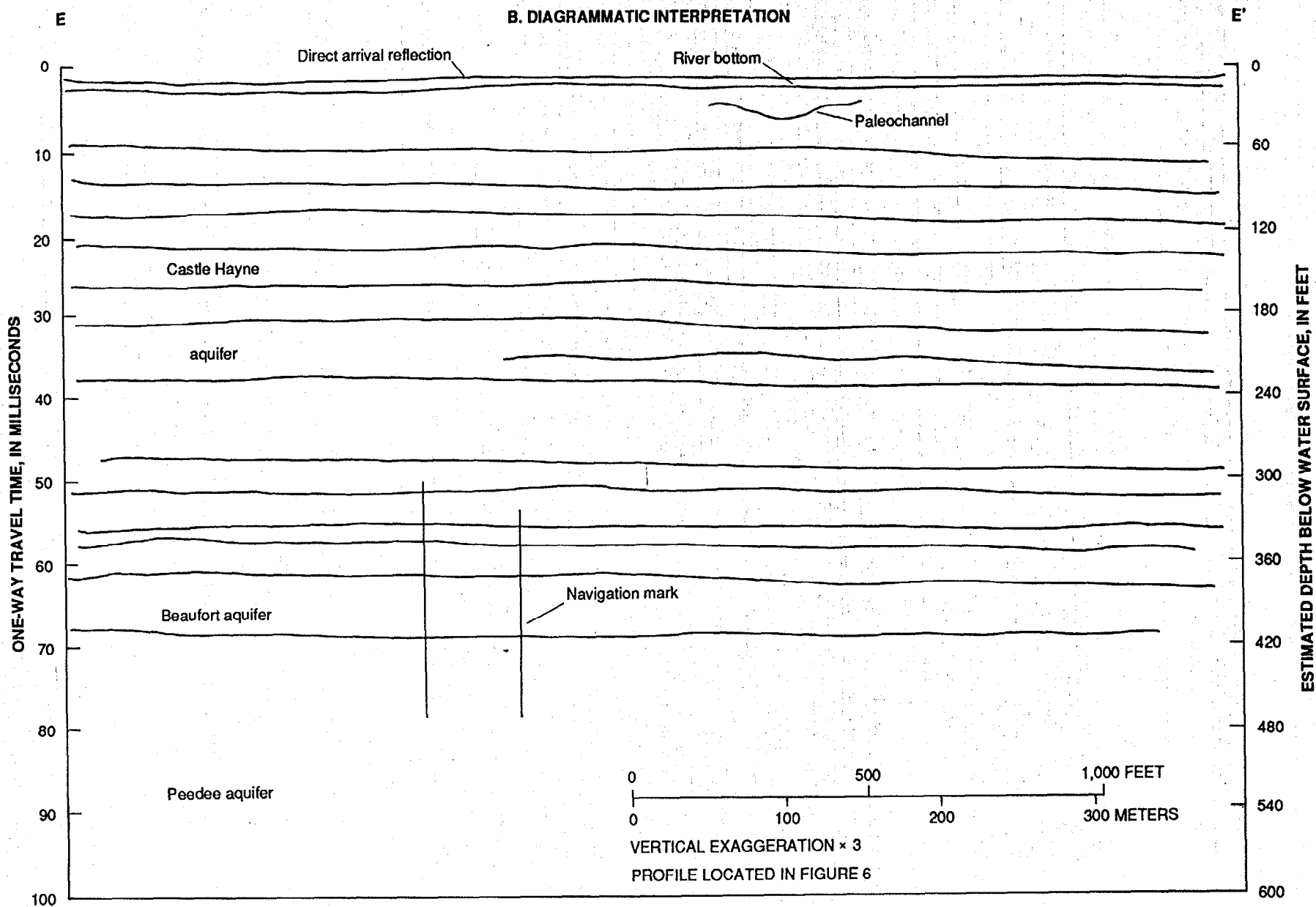
Figure 13.--(A) Seismic reflection record, and (B) diagrammatic interpretation for profile segment E-E'.
