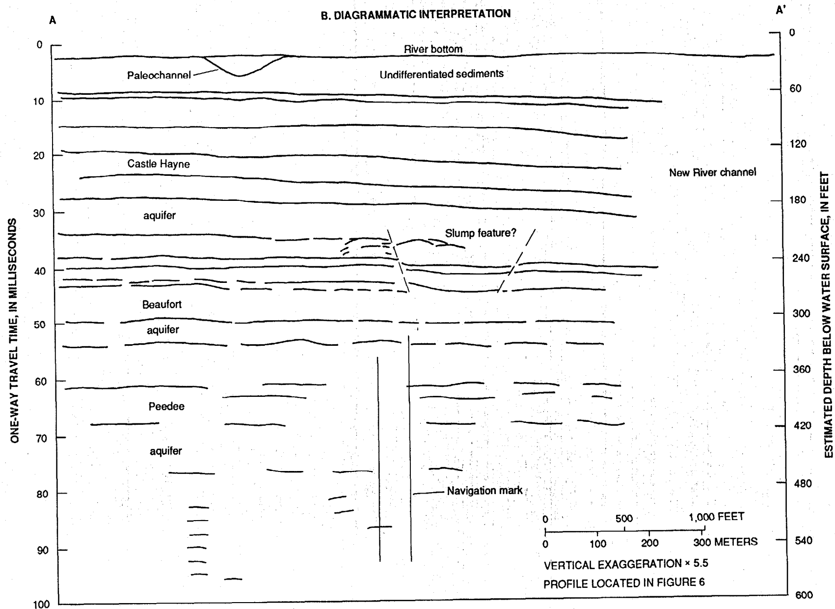
Figure 9.--(A) Seismic reflection record, and (B) diagrammatic interpretation for profile segment A-A'.
