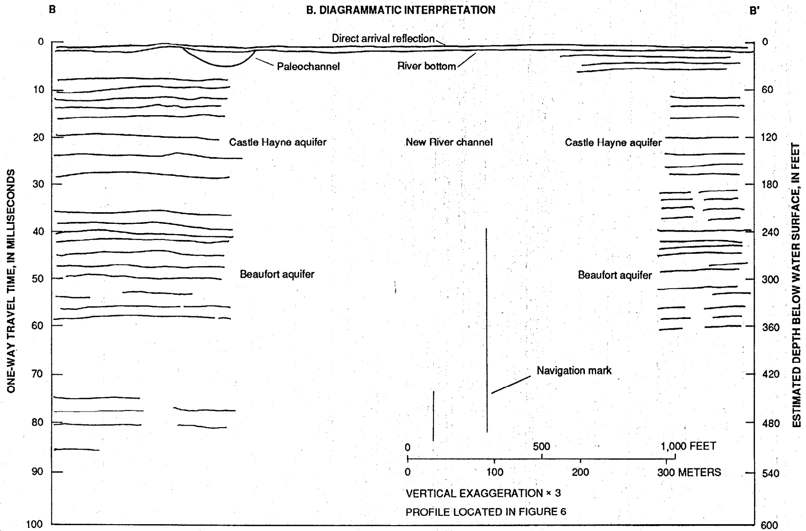
Figure 10.--(A) Seismic reflection record, and (B) diagrammatic interpretation for profile segment B-B'.
