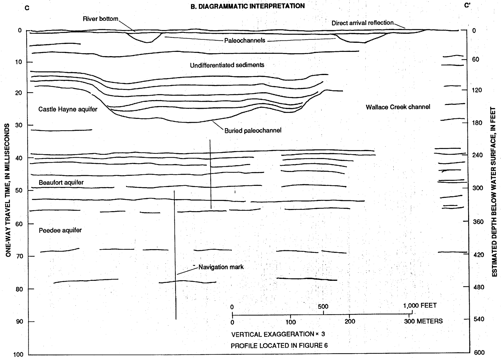
Figure 11.--(A) Seismic reflection record, and (B) diagrammatic interpretation for profile segment C-C + .
