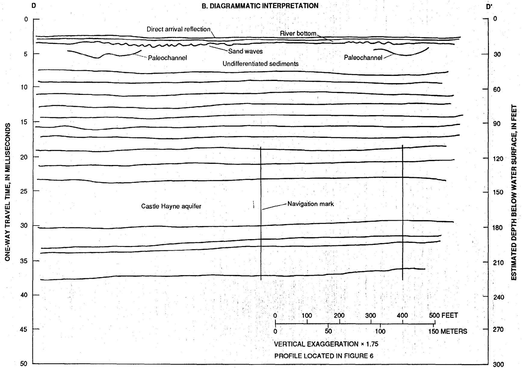
Figure 12.--(A) Seismic reflection record, and (B) diagrammatic interpretation for profile segment D-D'.
