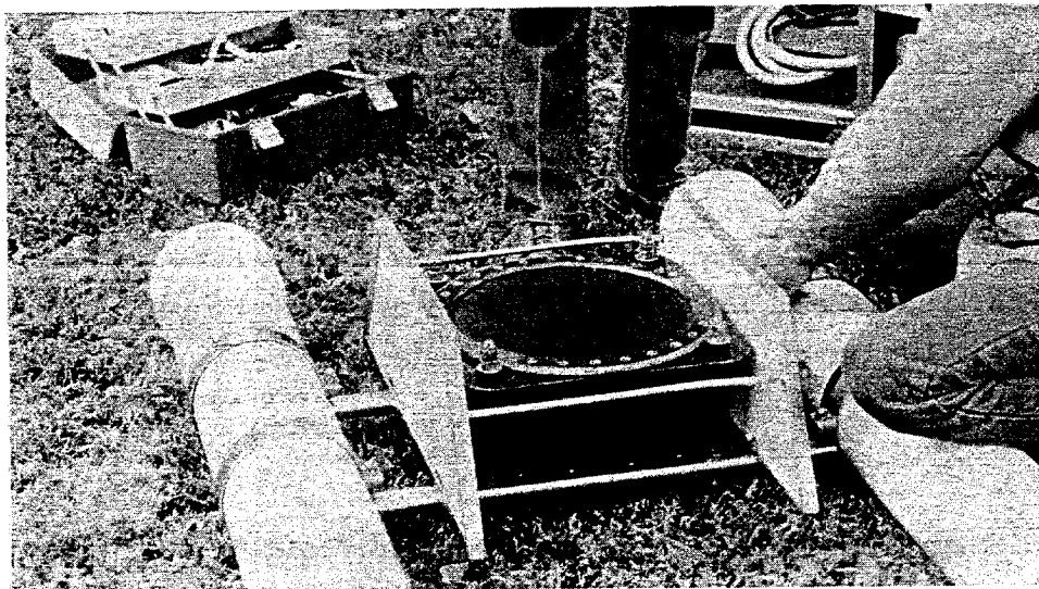
Figure 5.--The acoustic-source catamaran.
