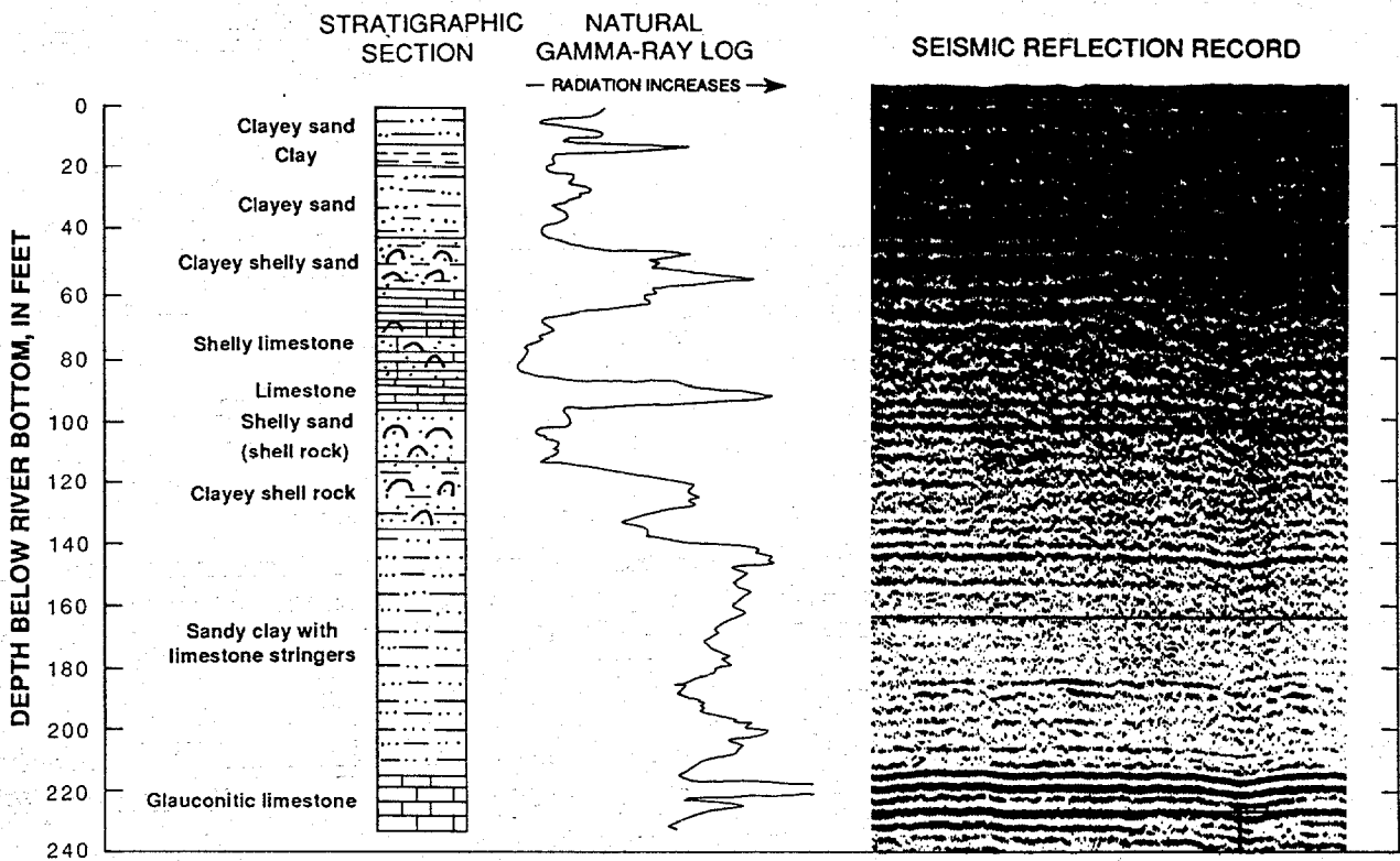
Figure 7.--Well log, stratigraphic, and seismic reflection record correlations made at well site 2.
