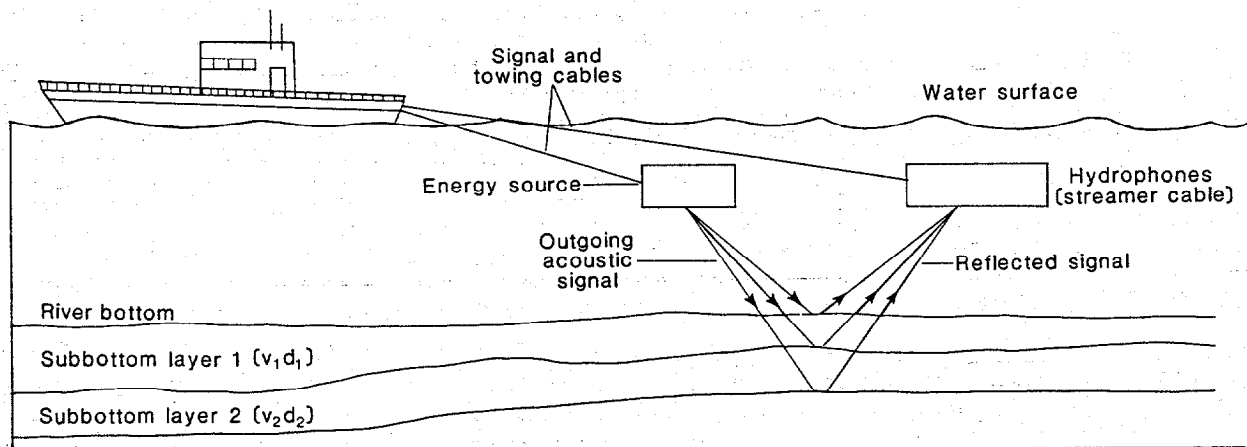
Figure 2.--Ray paths from acoustic source to hydrophones for single-channel seismic profiling.
