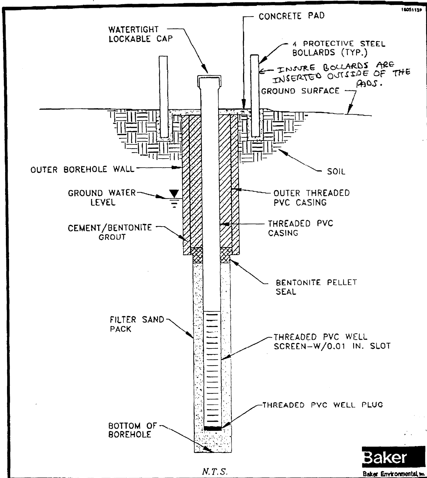
FIGURE 5-2 TYPICAL DEEP ABOVE GRADE TYPE III GROUNDWATER MONITORING WELL CONSTRUCTION DIAGRAM SITES 1, 28 AND 30
