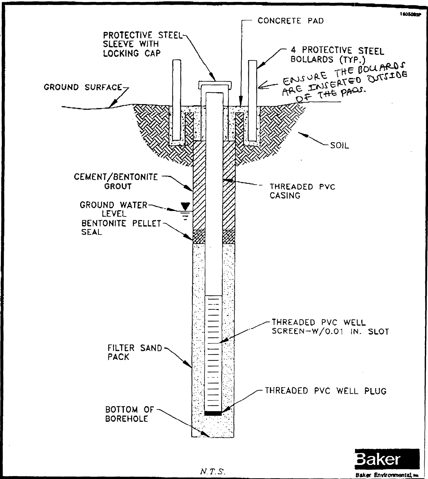
FIGURE 5-1 TYPICAL SHALLOW AND DEEP ABOVE GRADE TYPE II GROUNDWATER MONITORING WELL CONSTRUCTION DIAGRAM SITES 1, 28, AND 30
